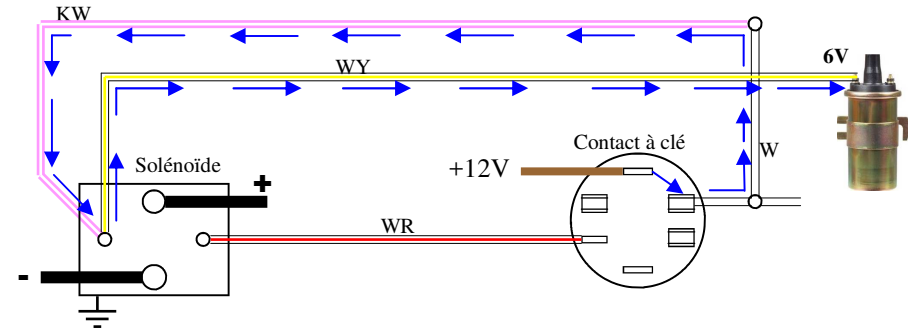
Schéma A position marche (Ignition)
