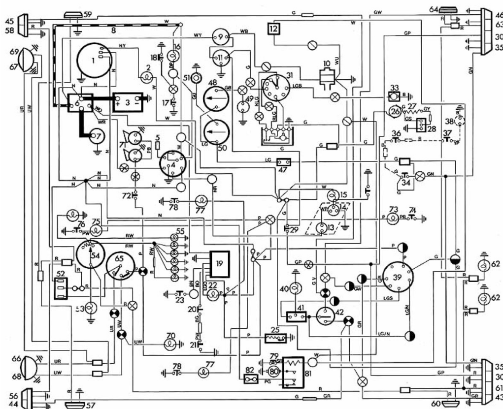
Fig. 10.66 Wiring diagram for N. American LHD Spitfire 1500 from commission number FM95001
